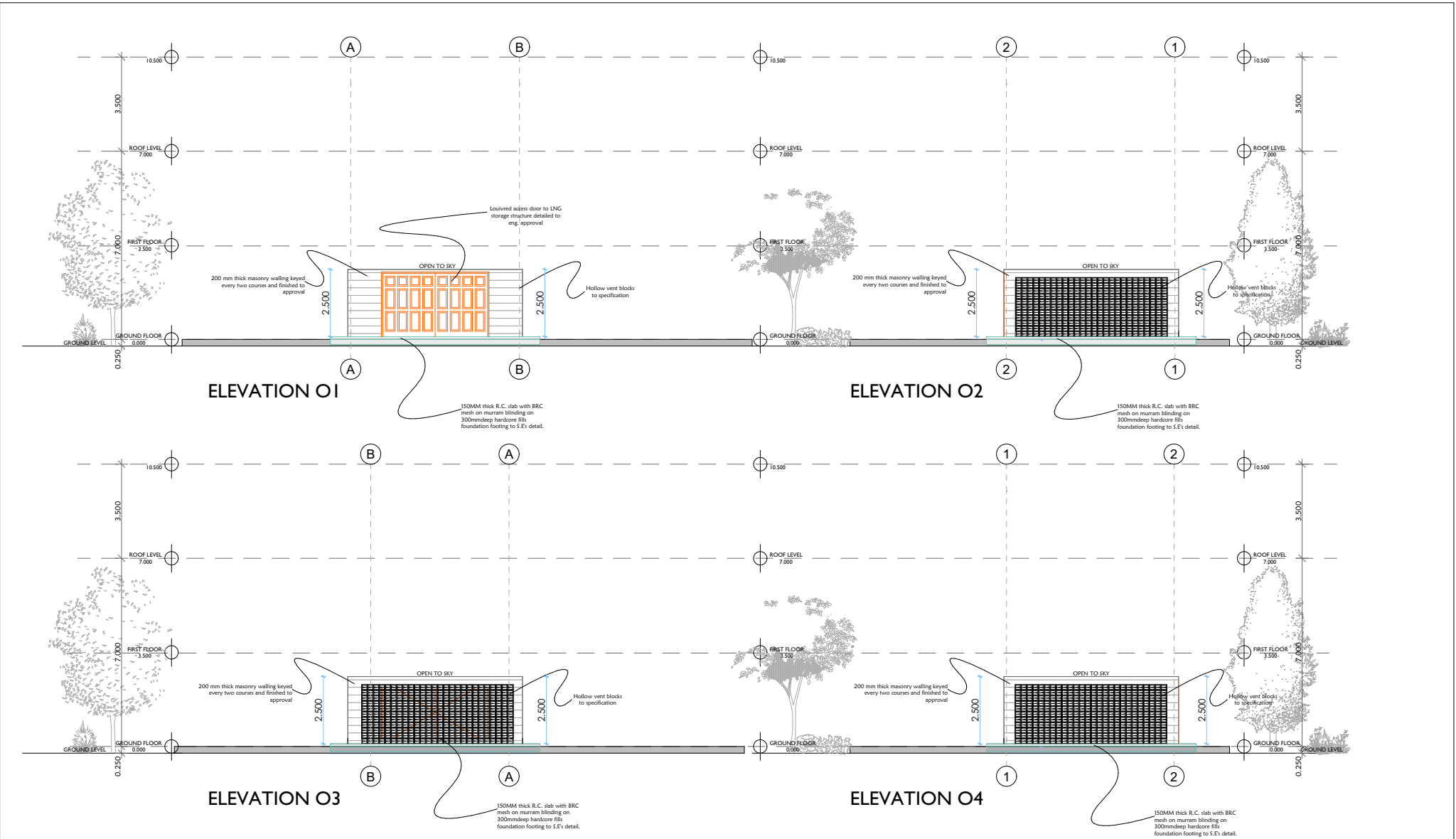
TYPICAL ELEVATIONS
